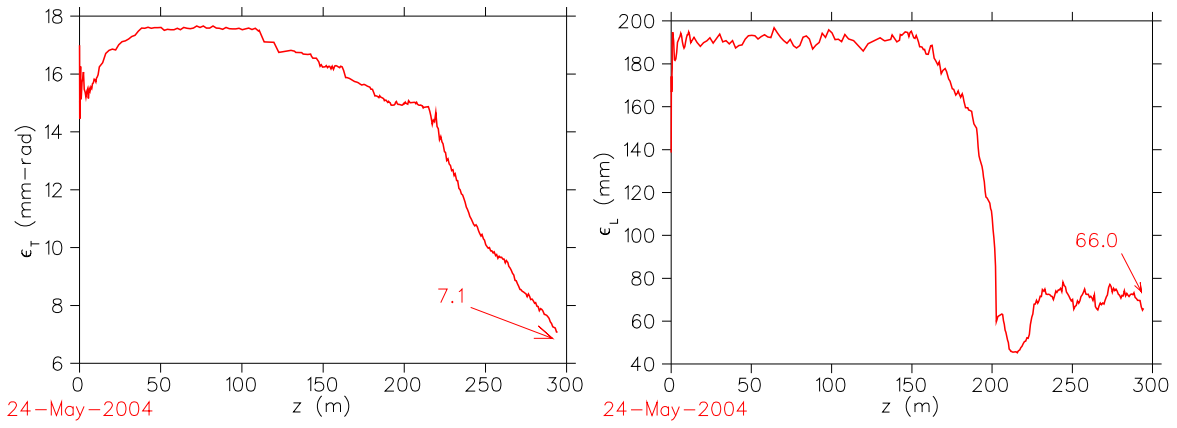
FIG. 42: (Color) Normalized transverse emittance (left) and longitudinal emittance (right) along the front-end for a momentum cut 0.1 \leq p \leq 0.3 GeV/c.
