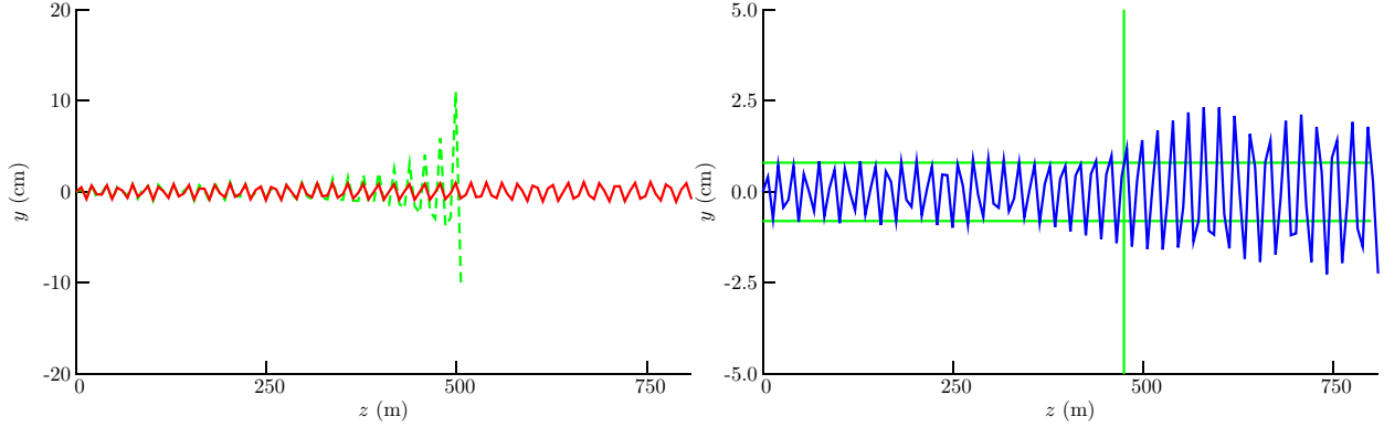
FIG. 56: (Color) Tracking of a particle at the edge of the acceptance with uniform acceleration in the 5–10 GeV reference lattice. On the left, the dashed line is without any body sextupole, and the solid line is with the corrected body sextupole. On the right, a smaller integrated sextupole correction is used (40% instead of 68%), and significant emittance growth is observed.
