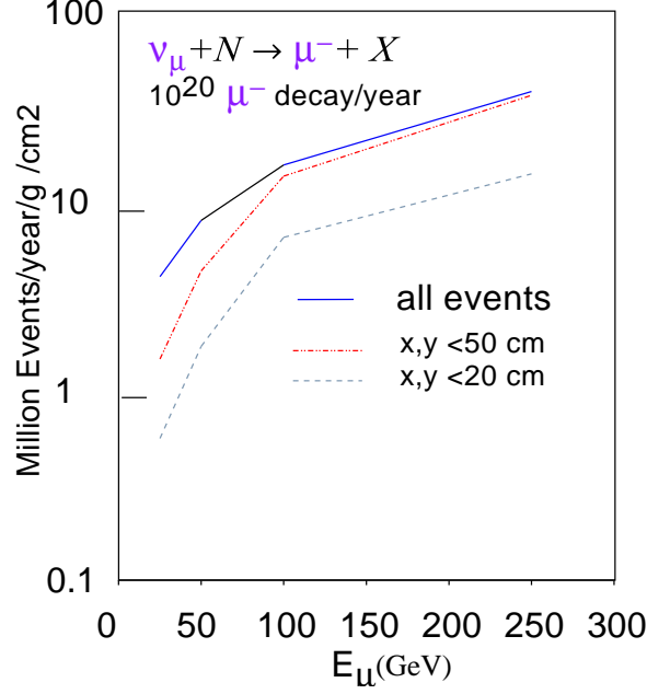
FIG. 17: (Color) Events per year and per \text{g}/\text{cm}^2 at a near detector as a function of muon beam energy in GeV. The solid curves indicate all events, the dashed and dotted curves show the effects of radial position cuts.
