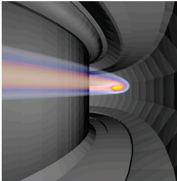
Computer-generated 3D view of runaway electrons in DIII-D based on high speed 2D images of synchrotron emission from electrons traveling near the speed of light inside the tokamak.
