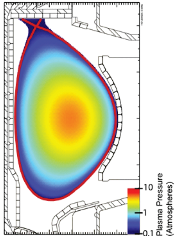
Figure 1: Surfaces of constant plasma pressure in the cross-section of the C-Mod tokamak for an I-mode plasma. In the hottest core region, the pressure exceeds 4 atmospheres. The volume average pressure is over 1.5 atmospheres, more than 50 percent of the central pressure expected in the ITER device, and close to the current tokamak world record of 1.8 atmospheres, also attained on C-Mod.
