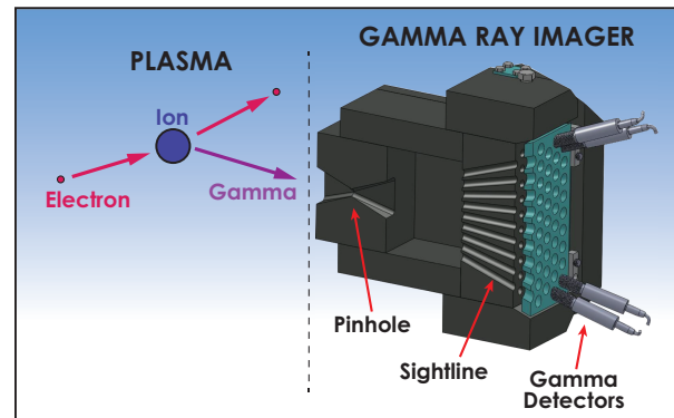
Figure 1. Gamma Ray Camera: Cross section of gamma ray imager and illustration of emission from energetic electrons (Image by General Atomics).
