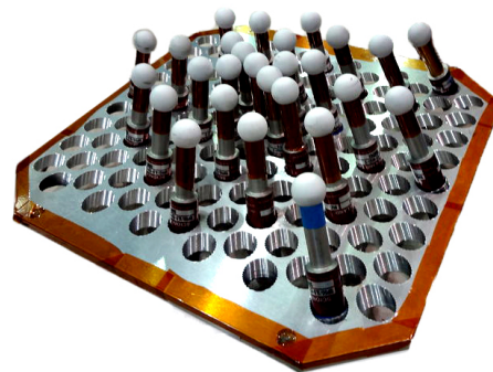
Figure 2. Gamma Ray Detectors: Each pixel of the camera is an individual detector pictured above. These are arranged to look into the plasma and focus on the hottest part of the plasma.
