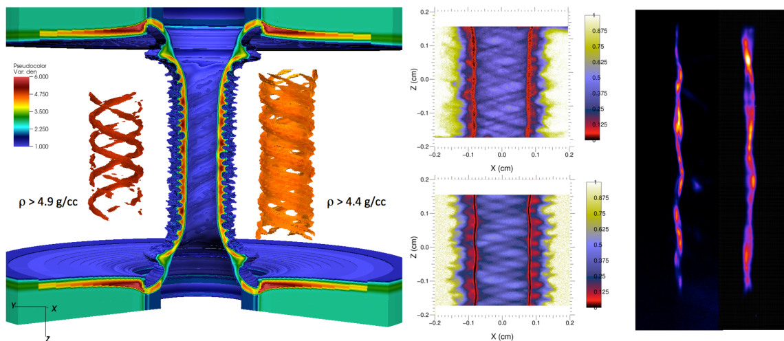
Figure 1: (Left) Simulated density profiles highlighting the helical instability growth in the Z-pinch; (Center) Experimental [top] and synthetic [bottom] x-ray transmission radiographs of the helical perturbation in the liner during the implosion; (Right) Experimental [left] and synthetic [right] x-ray emission images of the hot plasma at stagnation and peak fusion burn.
