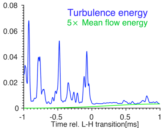
Figure 1: The turbulence and mean flow energies as a function of the time relative to the start of H-mode.
