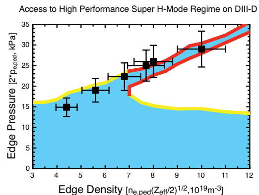
Figure 1: Safe passage of the DIII-D experiment (black symbols) to high edge pressure (red-bounded Super-H Mode region) requires precise navigation through operating conditions. [Courtesy of General Atomics]
